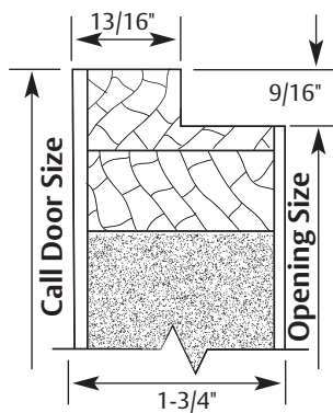
Typical Rabbet
