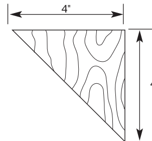
Shelf Bracket
